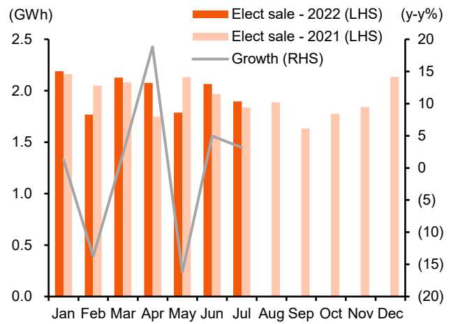
Ex 4: Electricity Output From Its Solar Farms
